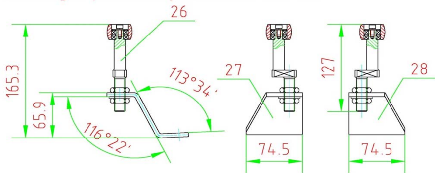
Slider Mechanism (L) (The right piece is symmetrical with it)
